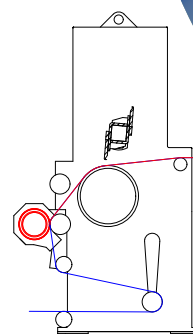
COMBINED COATING HEAD WITH SCREEN ROLL AND BLADE
