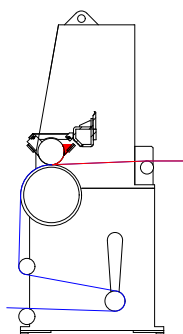
COMBINED COATING HEAD WITH BLADE AND ENGRAVED ROLL
