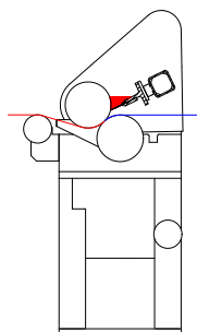
ROLL COATING HEAD
